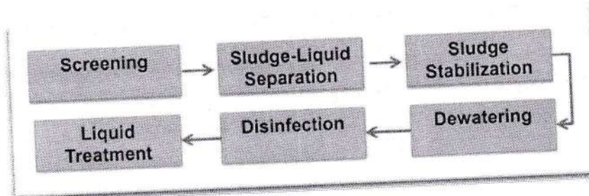
FLOW DIAGRAM FOR A FSTP
